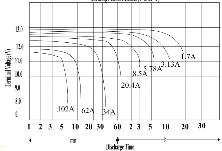
Discharge Characteristics (0 °C, 32 °F)
