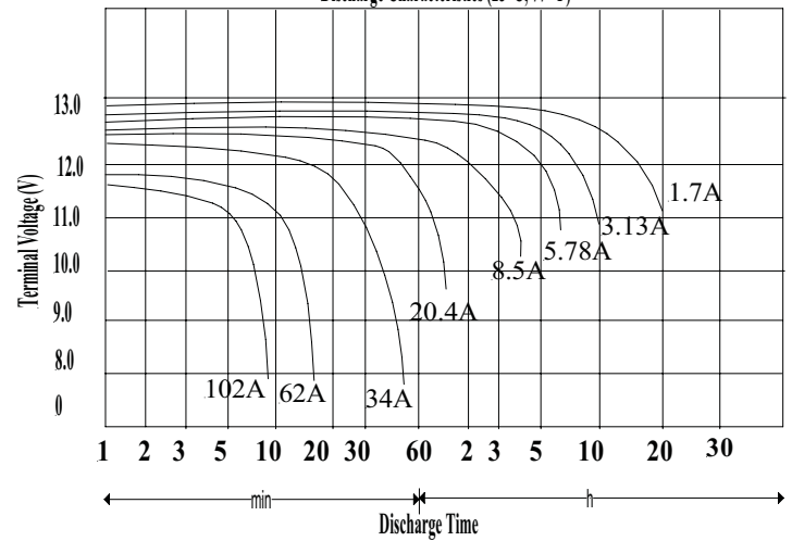
Discharge Characteristics (25 °C, 77 °F)
