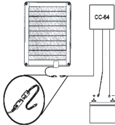
SAE Connector for easy connection to FLX Modules
