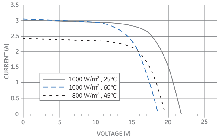
Typical I-V Curve for GEPV-045 Module
